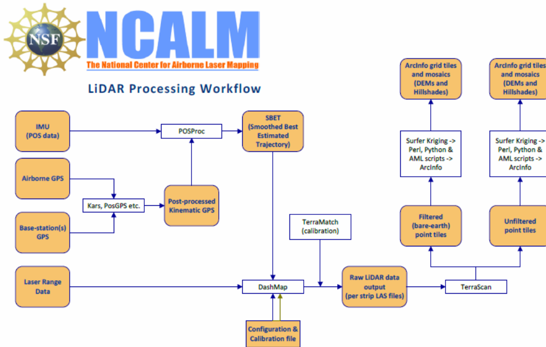
Figure 2: NCALM LiDAR processing workflow
