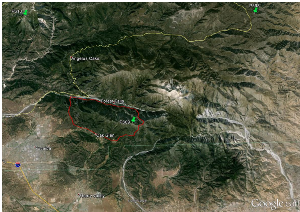
Figure 1 – Shape and location of survey polygon (red). P598, P613, and P609 indicate locations of GPS reference stations. (Google Earth).
