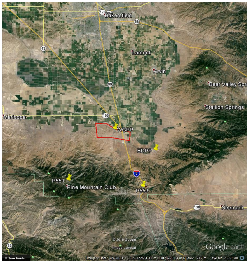
Figure 1 – Shape and location of survey polygon (red). P551, P553, EDPP and WGPP indicate locations of GPS reference stations. (Google Earth).
