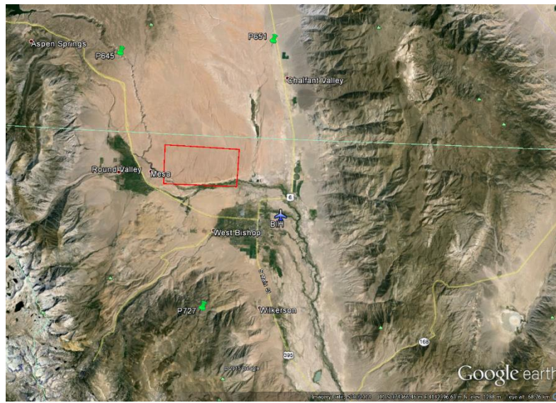
Figure 1 – Shape and location of survey polygon (red). P645, P651, P727 and BIH indicate locations of GPS reference stations. (Google Earth).
