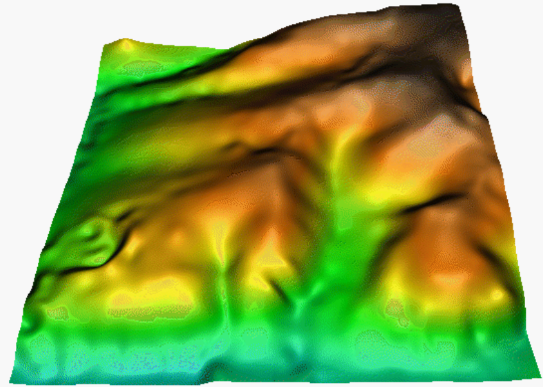
Regularized Spline with Tension and smoothing (RST)
