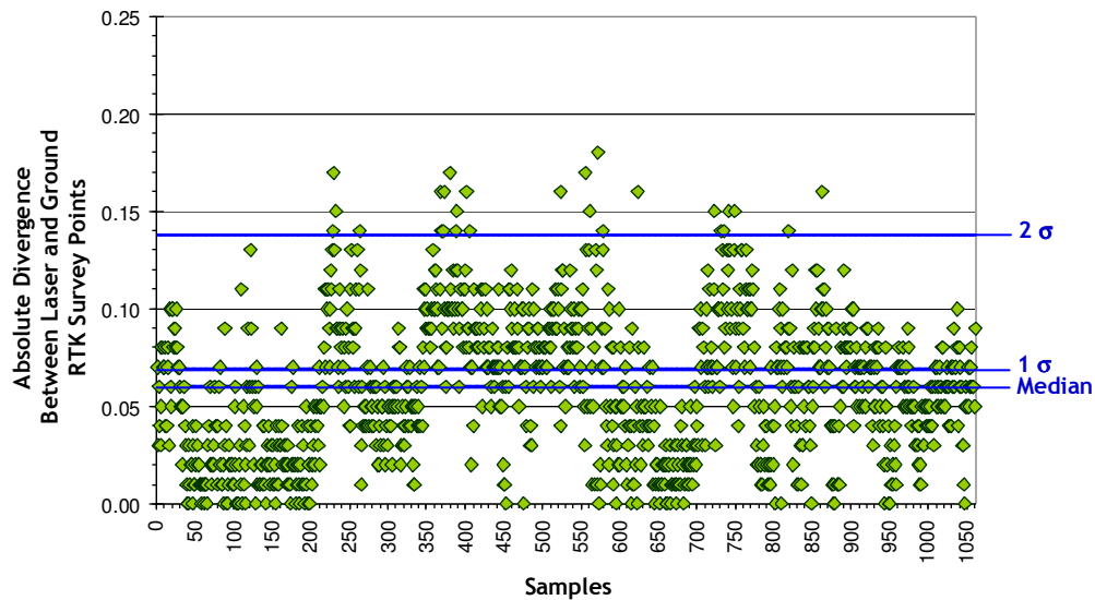
Figure 10. Point Absolute Deviation Statistics
