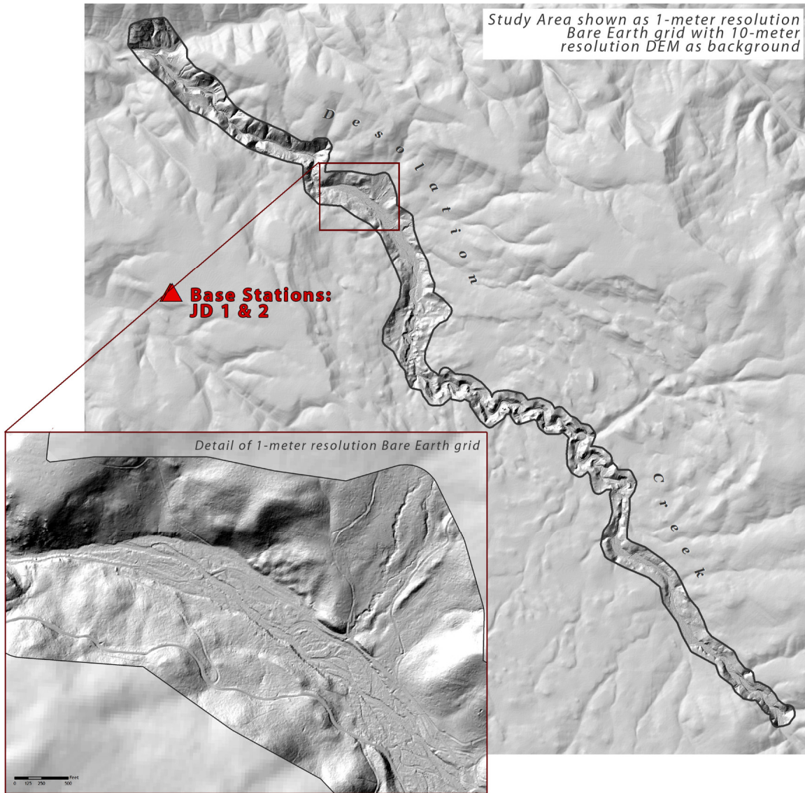
Figure 3. Locations of Base Stations and RTK Survey Point Collection: Desolation Creek Study Area, Base Stations JD 1 & 2.
