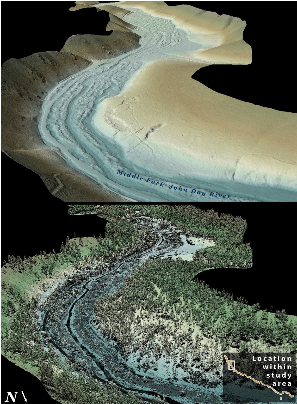
Figure 15. 3-d oblique view of LiDAR-derived surfaces in bins MF03-MF04 of the Middle Fork John Day River Study Area (top image derived from ground-classified points, bottom image derived from all points).
