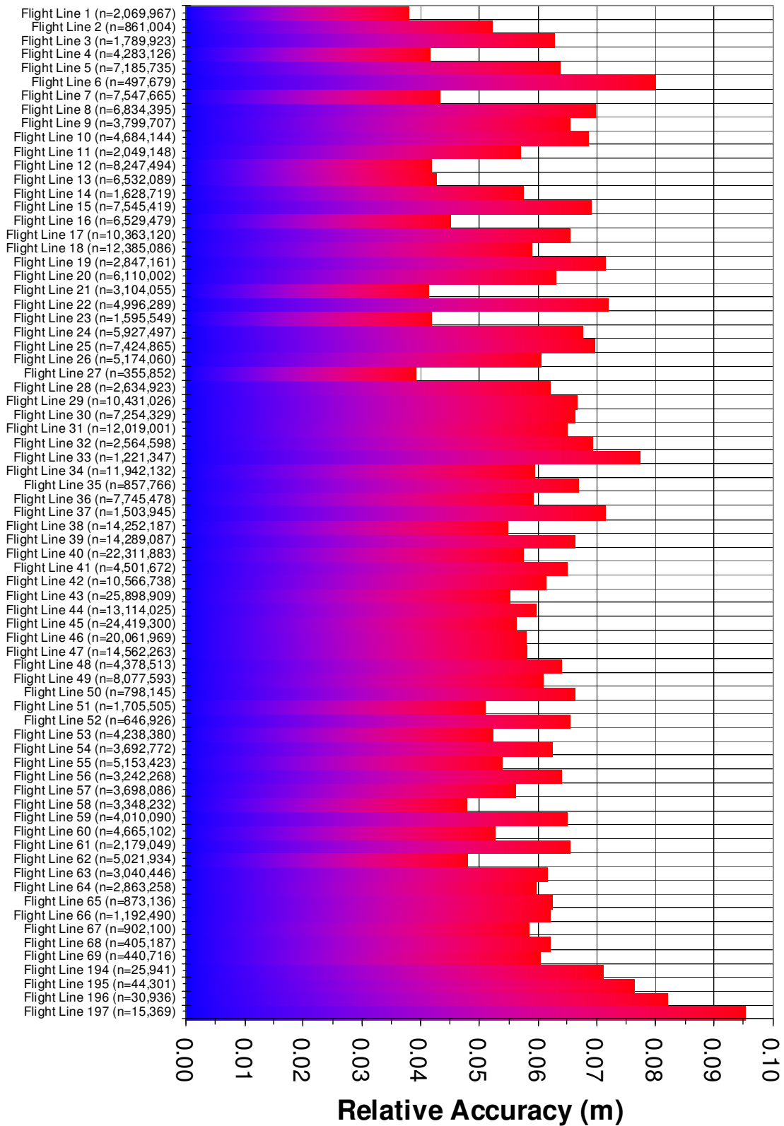
Figure 6. Relative accuracy per flight line with overlapping point totals listed as 'n'.
