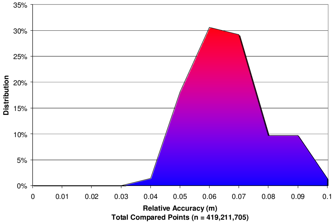
Figure 8. Statistical relative accuracies.
