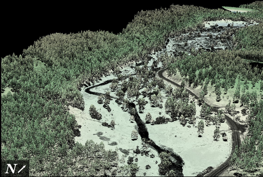
LiDAR-Derived Surface: Point Cloud of all Laser Returns, Shown by Intensity and Elevation, Middle Fork John Day River Study Area
