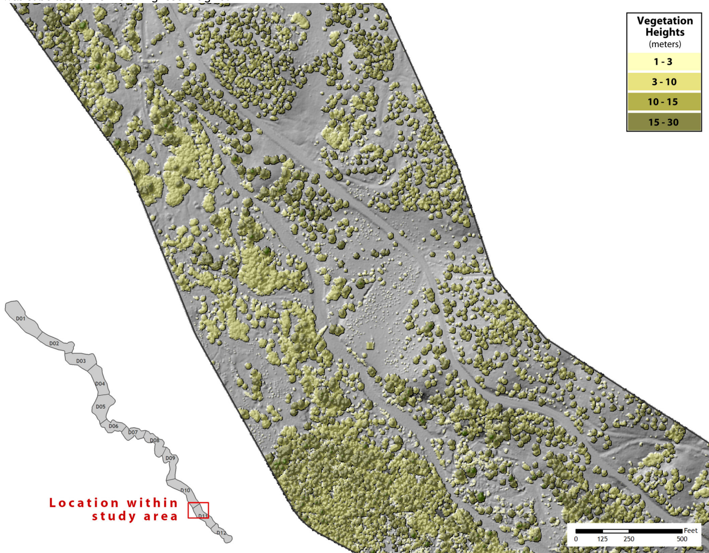
Figure 12. The Highest Hit 1-meter resolution ESRI grid showing detail in Desolation Creek Study Area (bins D10-D11). To calculate vegetation heights, the Bare Earth grid was subtracted from the Highest Hit grid.
