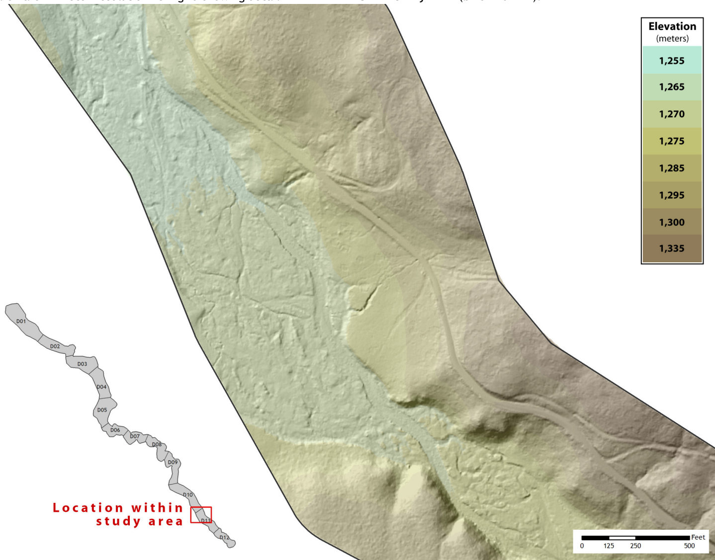
Figure 11. Bare Earth 1-meter resolution ESRI grid showing detail in Desolation Creek Study Area (bins D10-D11).
