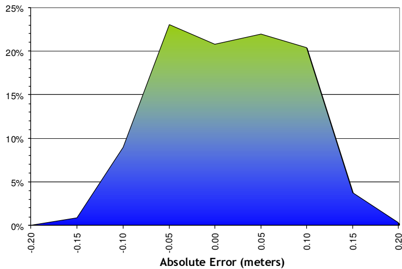
Figure 10. Point Absolute Deviation Statistics
