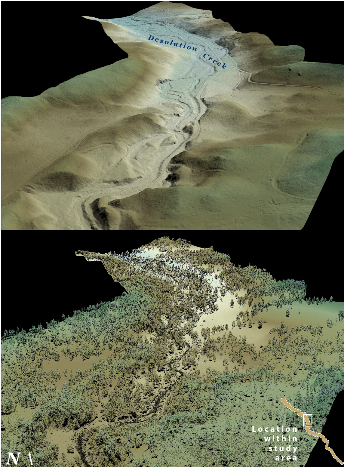
Figure 14. 3-d oblique view of LiDAR-derived surfaces in bins D04-D05 of the Desolation Creek Study Area (top image derived from ground-classified points, bottom image derived from all points).
