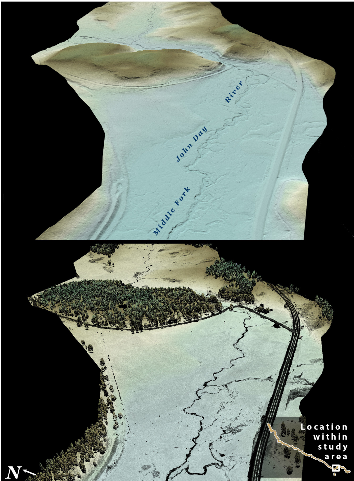
Figure 16. 3-d oblique view of LiDAR-derived surfaces in bins MF23-MF24 of the Middle Fork John Day River Study Area (top image derived from ground-classified points, bottom image derived from all points).
