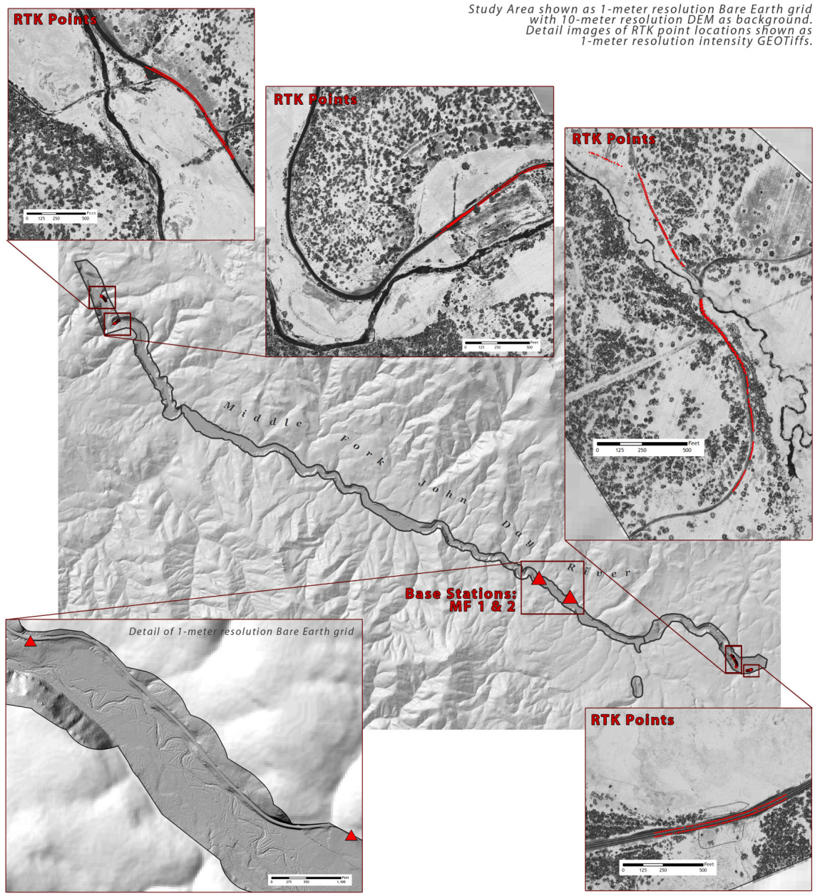
Figure 4. Locations of Base Stations and RTK Survey Point Collection in the Middle Fork John Day Study Area, Base Stations MF 1 & 2, 1061 RTK Points.
